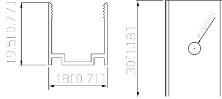
Fixed Buckle
